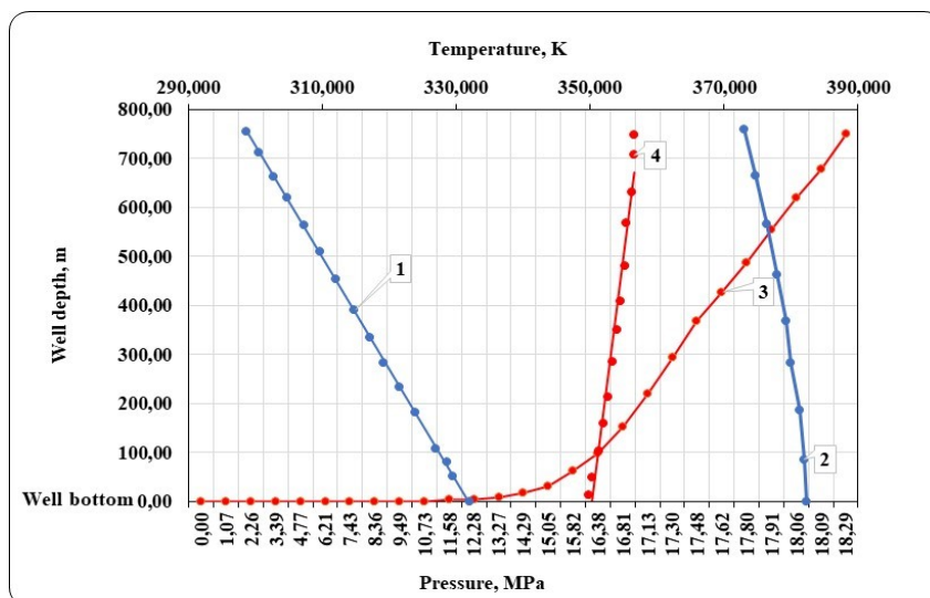
Fig. 2. Distribution of fluid temperature and pressure profiles in the well: 1 – oil pressure; 2 – water pressure; 3 – oil temperature; 4 – water temperature.
