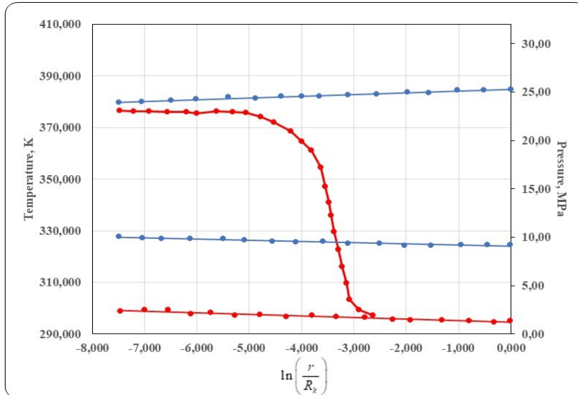
Fig. 1. Distribution of fluid temperature and pressure in formation:
